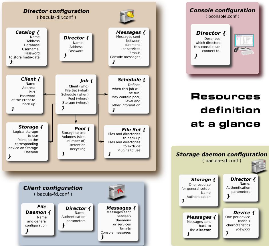
Figure 22.1: Bacula Objects
