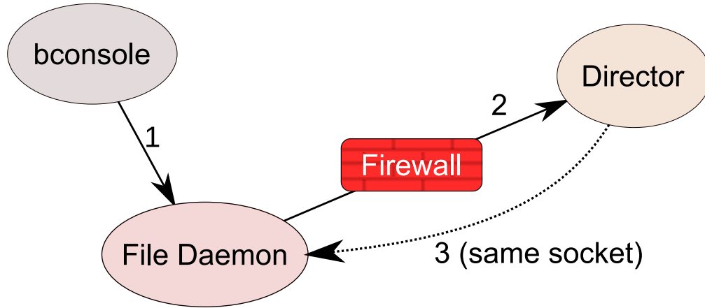
Figure 8.2: Client Initiated Backup Network Flow
