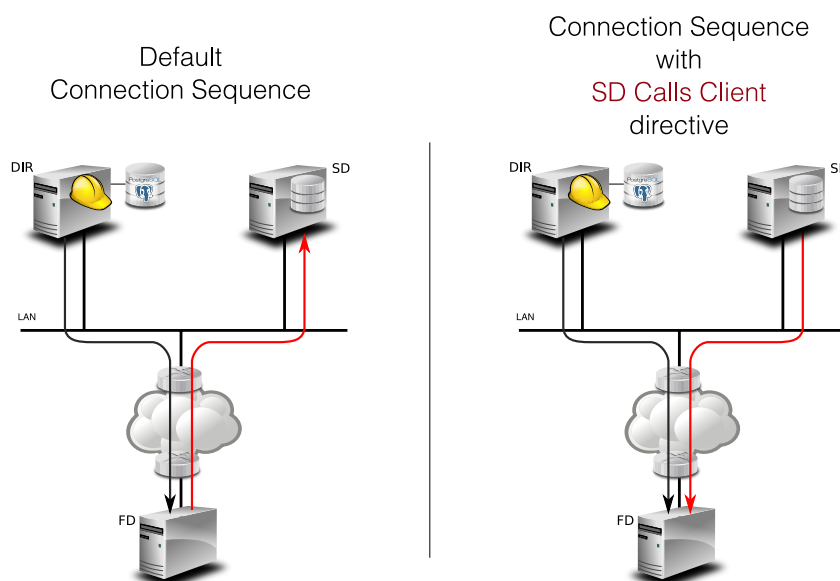
Figure 55.21: SD Calls Client
