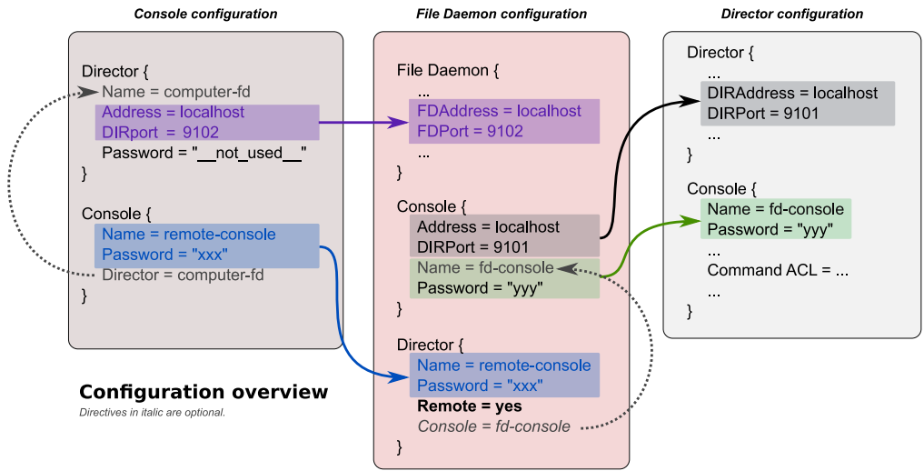
Figure 8.3: Relation Between Resources (bconsole)
