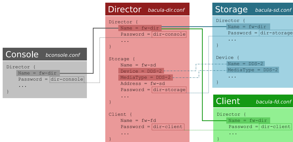
Figure 22.2: Configuration diagram
