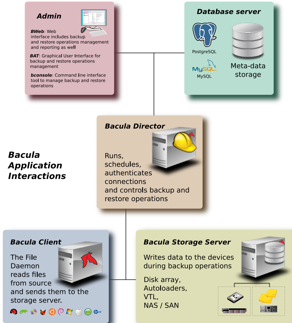
Figure 1.1: Bacula Applications
